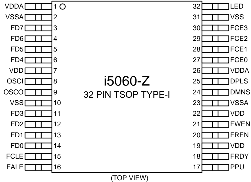
Figure 1. Pin configuration
